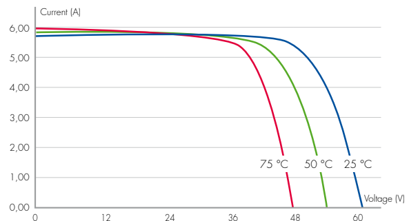
IU Curves at different temperature
