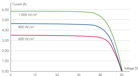
IU Curves at different irradiance
